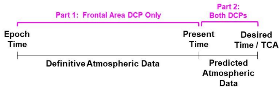
Figure N-8 Two-phase Application of Consider Parameters
