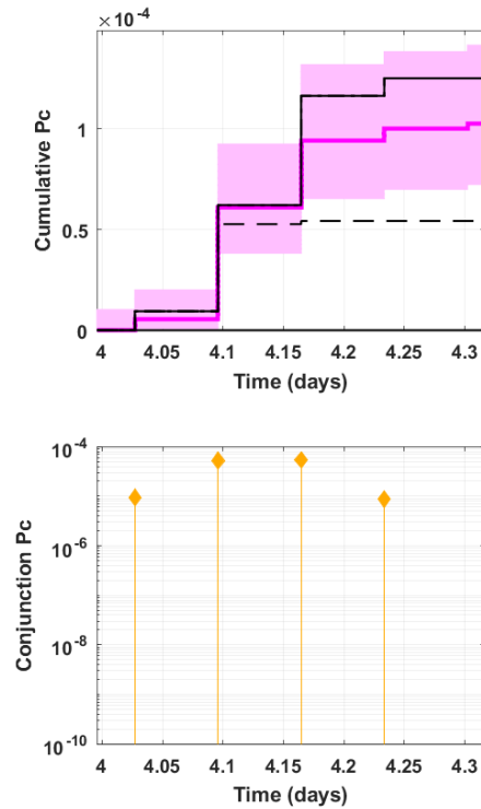
Figure N-10 Three-Dimensional N_c Temporal Risk Plot with Monte Carlo Result Overlay (in Pink)
