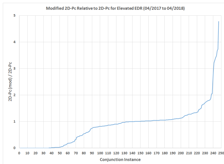
Figure N-9 Profiles of 250 Conjunctions with Primary and Secondary Satellites of Non-negligible Drag 11
