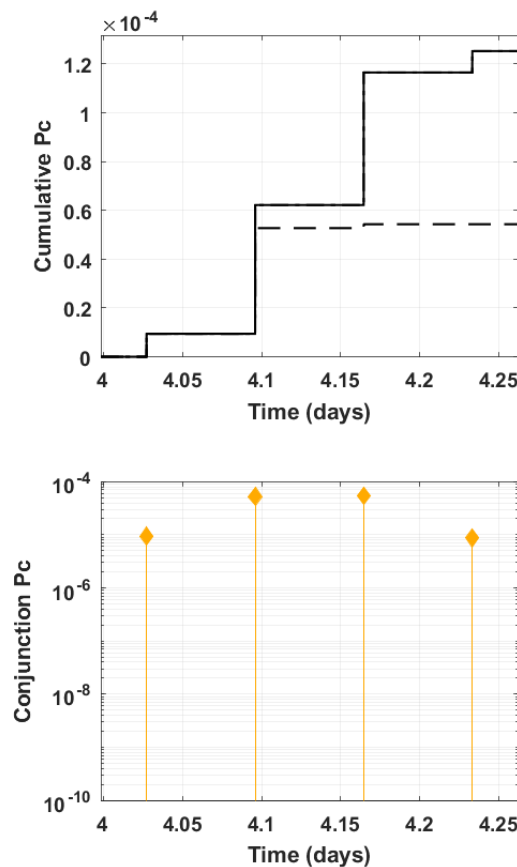
Figure N-6 Cumulative Three-Dimensional N_c Risk Over Four Repeating Conjunctions
