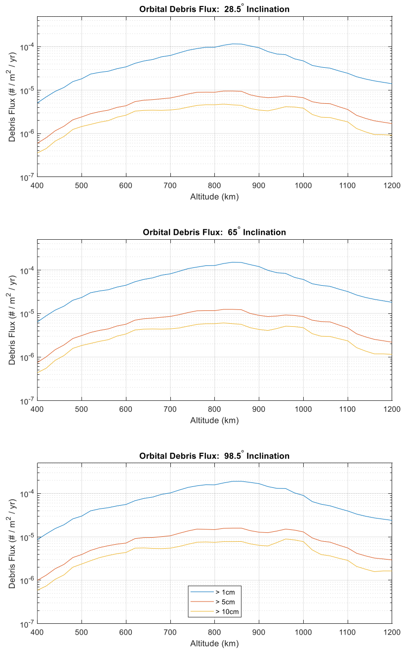
Figure G-1 Debris Flux as a Function of Orbit Inclination, Orbit Altitude, and Object Size
