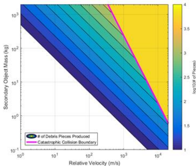
Figure O-1 Range of Debris Production Possibilities 16
