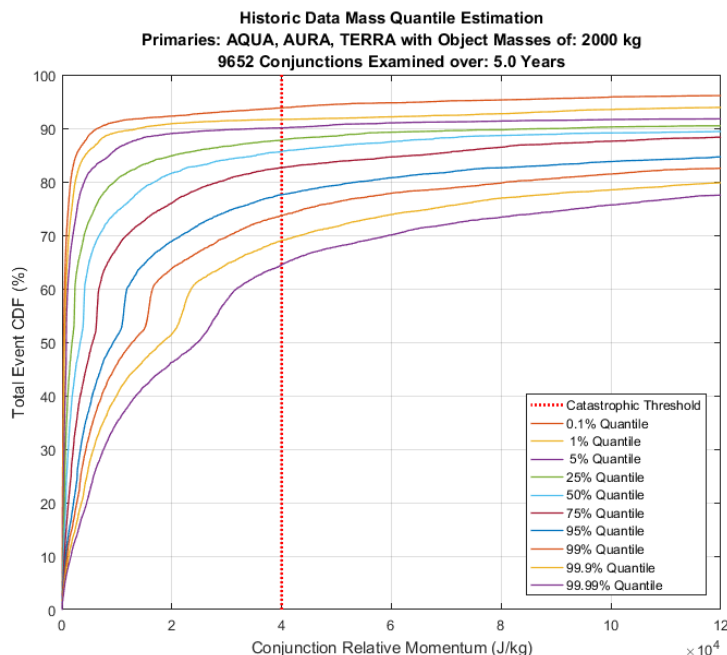
Figure O-3 Catastrophic/Non-Catastrophic Composition as a Function of Mass Quantile 18
