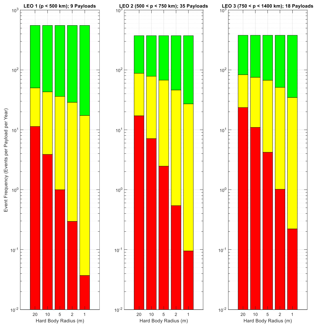
Figure F-1 CA Event Frequencies as a Function of Orbit Regime and Event Severity
