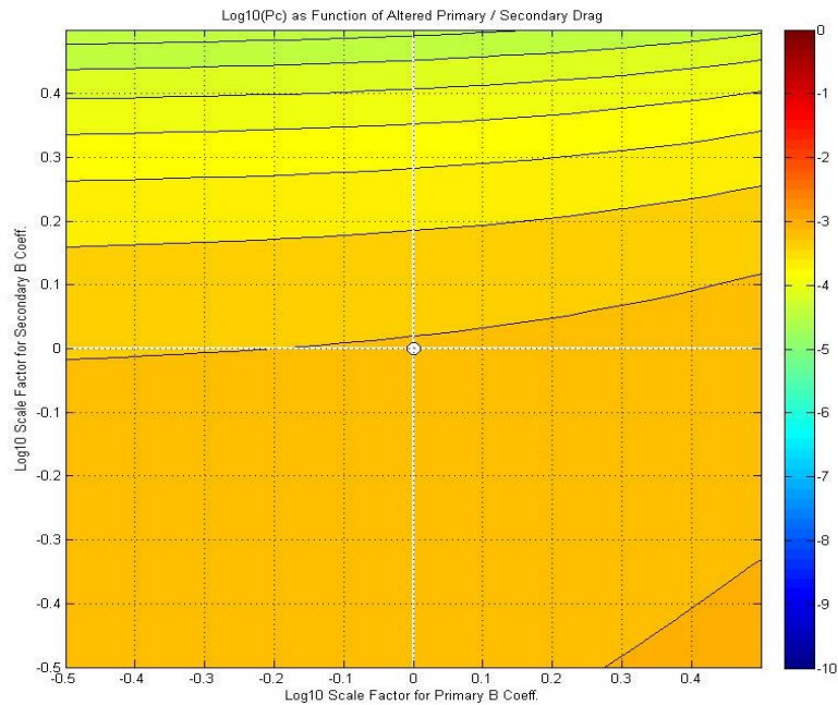
Figure P-1 SWTS Plot for Invariant Situation 19
