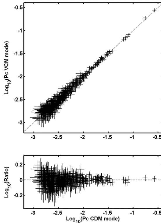
Figure N-12 Comparative Results of 373 High-Pc Conjunctions 12
