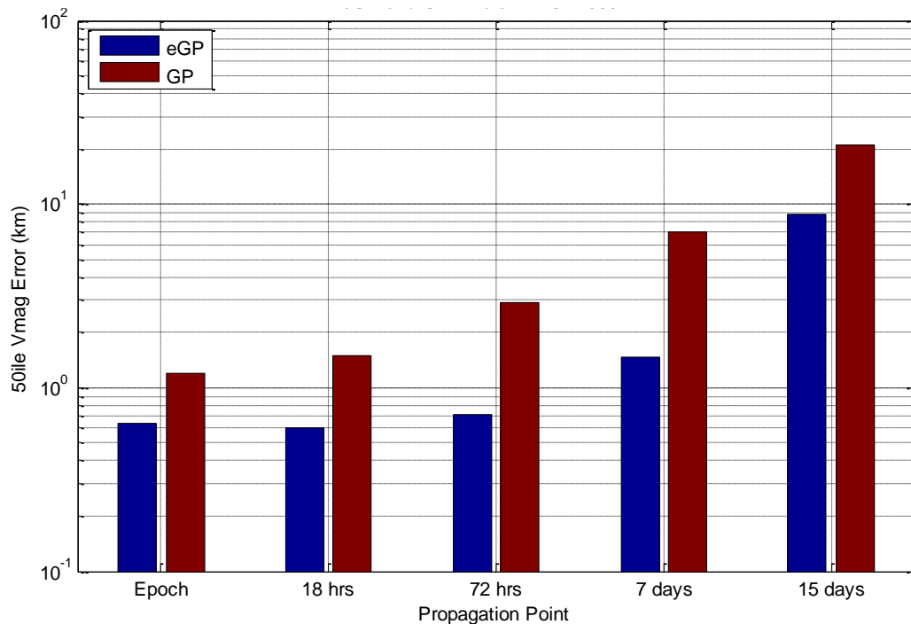
Figure E-2 eGP and Regular SGP4 Errors: LEO > 500 km (log scale) 8
