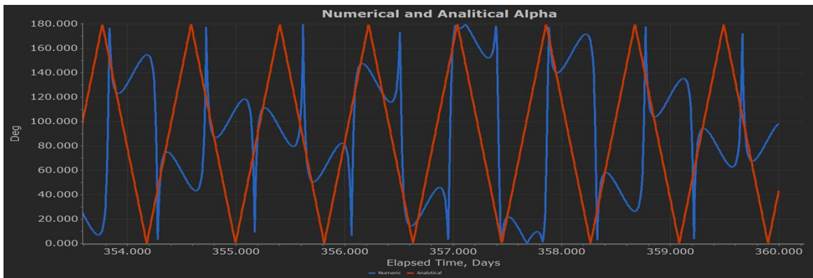
Figure H-2 Numerical vs. Analytical (Linear) \alpha for Highly Eccentric Orbit
