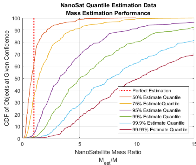
Figure O-2 Confidence in NanoSat Mass Ratio 17
