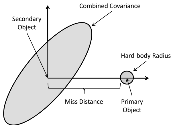
Figure N-4 Representation of the Conjunction Plane
