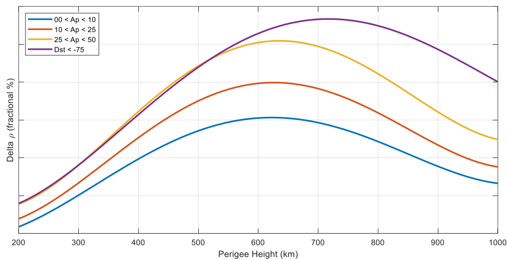
Figure N-7 Behavior of Relative Density Error by Perigee Height and Solar Activity
