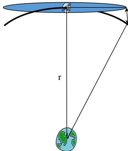
Figure N-11 Mismatch between Elongated In-track Covariances and Forced Cartesian Ellipsoidal Representation
