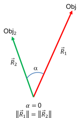
Figure H-1 Cartesian, Inertial, Earth-centered Position Vectors
