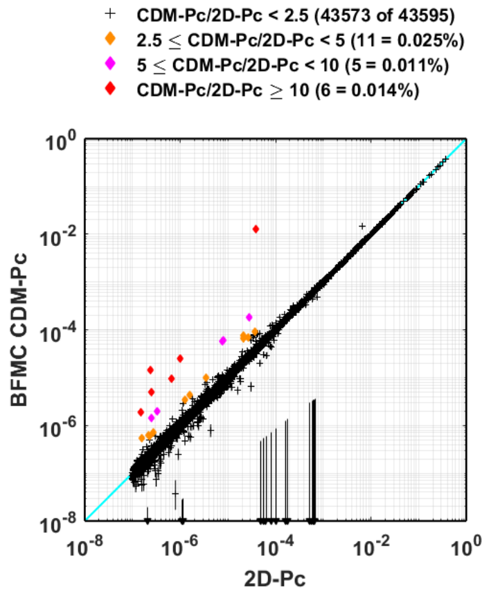
Figure N-13 Comparative Results of 44,000 Conjunction Events 13
