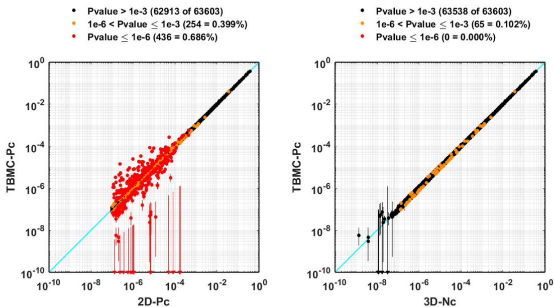
Figure N-5 Comparison of Monte Carlo Collision Probabilities with the Two-Dimensional P_c Method (left) and the Three-Dimensional N_c Method (right) for a Large Set of CARA Conjunctions
