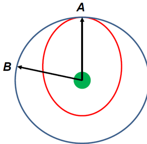
Figure H-3 Co-planar Orbits with One Circular and One Elliptical
